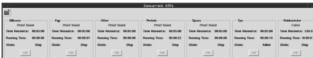
Fig. 4. Concurrent ATPs.
